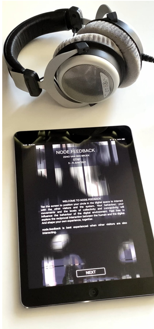
node.feedback, 2021
